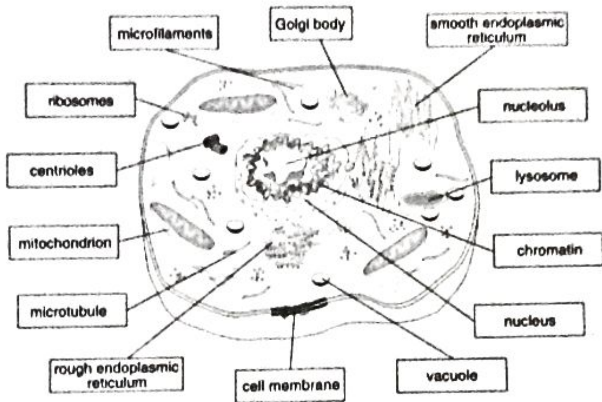
Animal Cell
