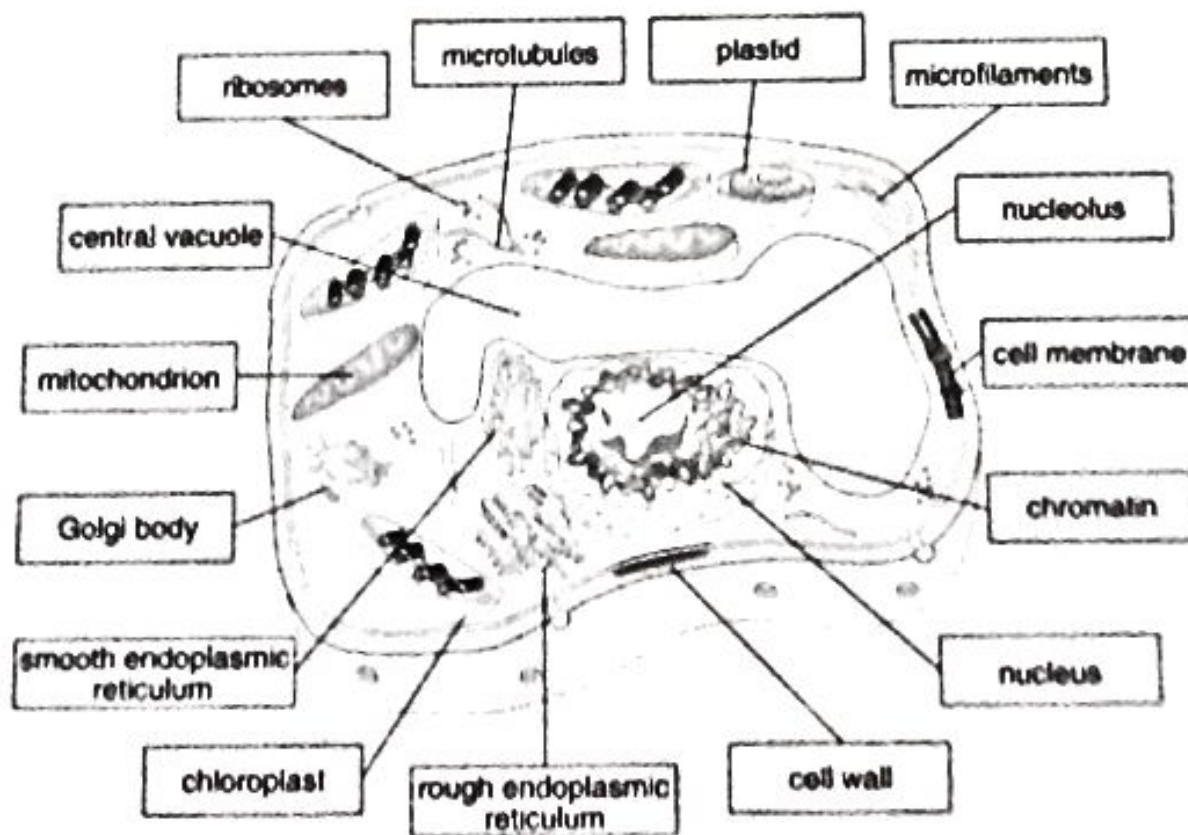
Plant Cell
